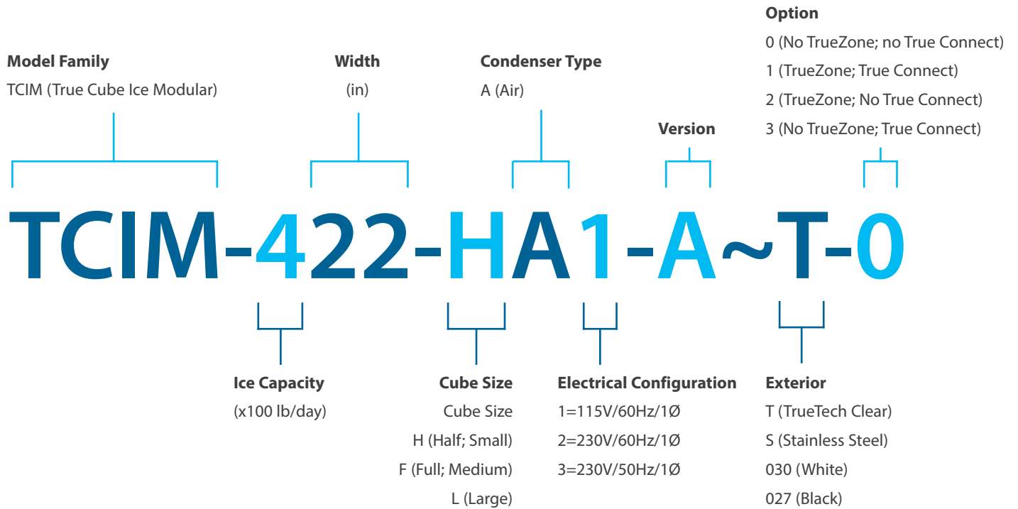
Fig. 2. TCIM model nomenclature diagram.
