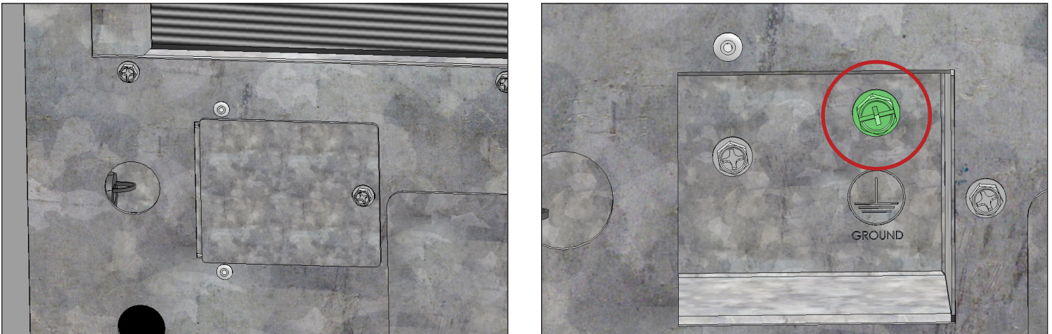
Fig. 3. Make the electrical connections inside the ice machine's junction box. Be sure to use strain reliefs. Always use the green grounding screw when making electrical connections.
