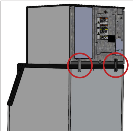
Fig. 1. Installed bin brackets.
