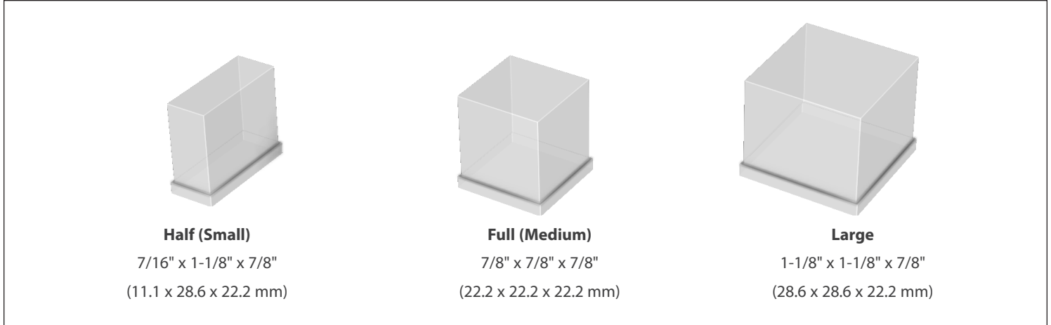
Fig. 1. Cube sizes and their dimensions.
