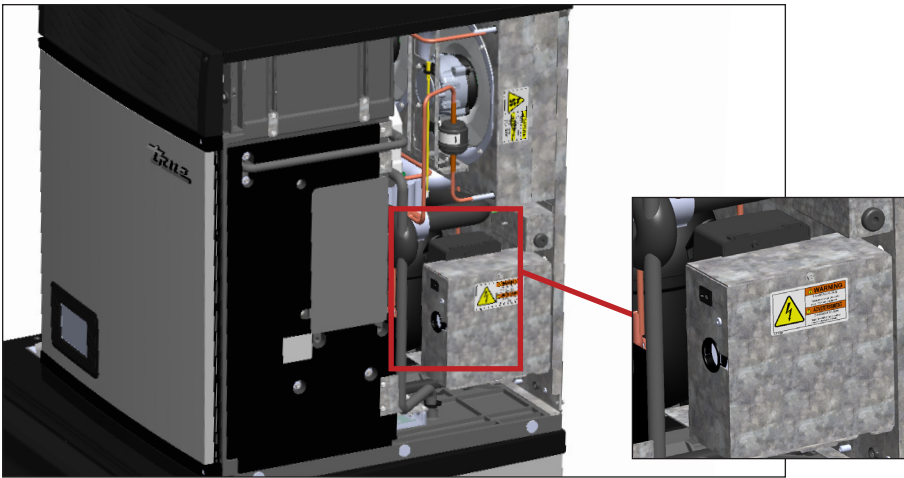
Fig. 2. Rocker switch location. Rocker switch disconnects power from the control board and front display; it DOES NOT disconnect power from the entire unit.
