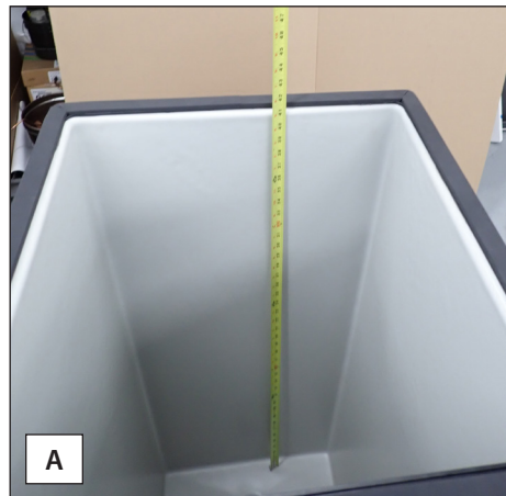
Fig. 2. Always measure the bin (A) or dispenser (B) for the ice level sensor before mounting the ice machine.
