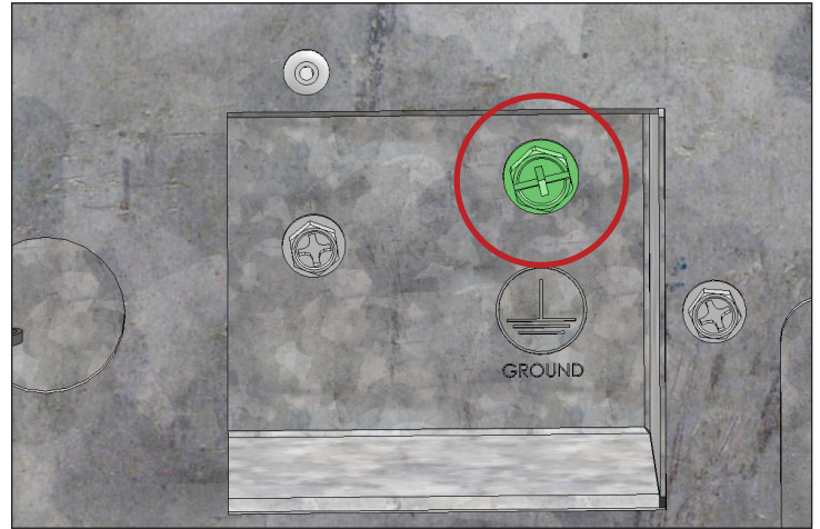
Fig. 3. Make the electrical connections inside the ice machine's junction box. Be sure to use strain reliefs. Always use the green grounding screw when making electrical connections.
