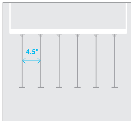
6 PEGS = 4.5" spacing
